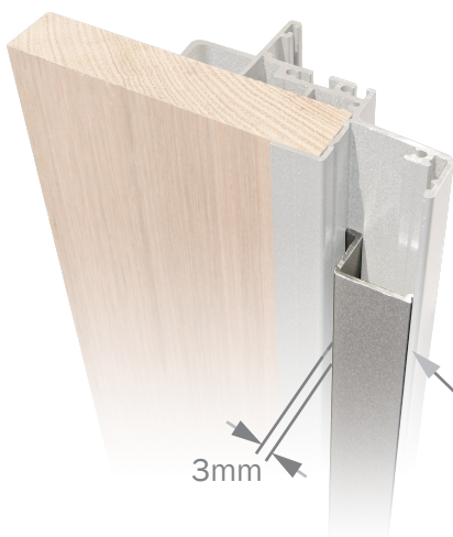
The optional external frame infill has a 15 x 3mm slot for flashing insertion (illustrated for clarity without secondary glazing)
